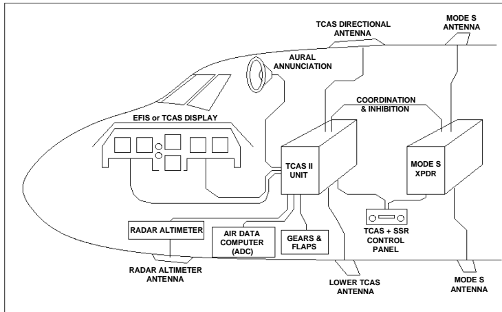
Figure 1: TCAS II block diagram
