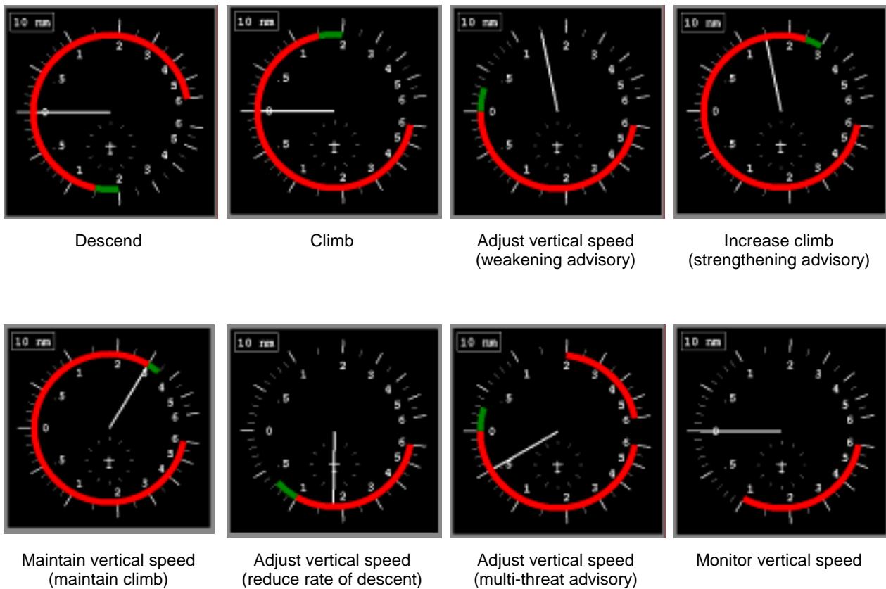
Figure 3: IVSI showing examples of RAs
