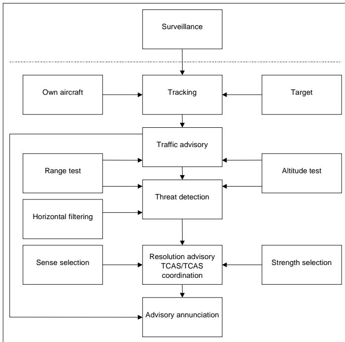
Figure 6: CAS logic functions
