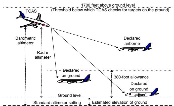
Figure 7: Target on-the-ground determination
