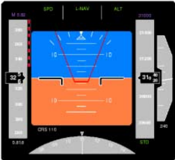
RA on the artificial horizon
