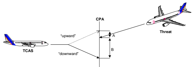
Figure 8: RA sense selection
